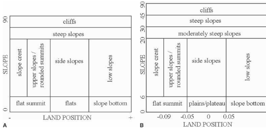
FIG. 2. Relationship between land position and slope parameters for the identification of landform units. 2a) TNC's base approach. 2b) Resulting relationships for Puerto Rico.
