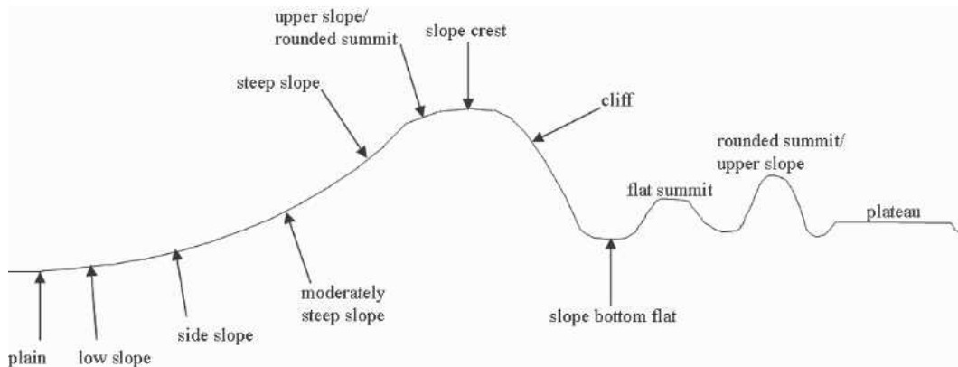
FIG. 3. Location of the different landforms across the landscape. Slope values are in real scale (adapted from TNC).
