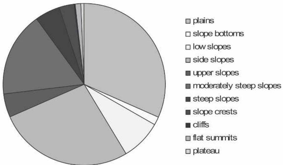
FIG. 4. Extent and proportion of the landforms in Puerto Rico.
