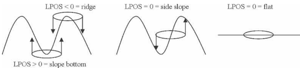
FIG. 1. Land position value (LPOS) for different situations along a slope (Source: TNC unpublished).
