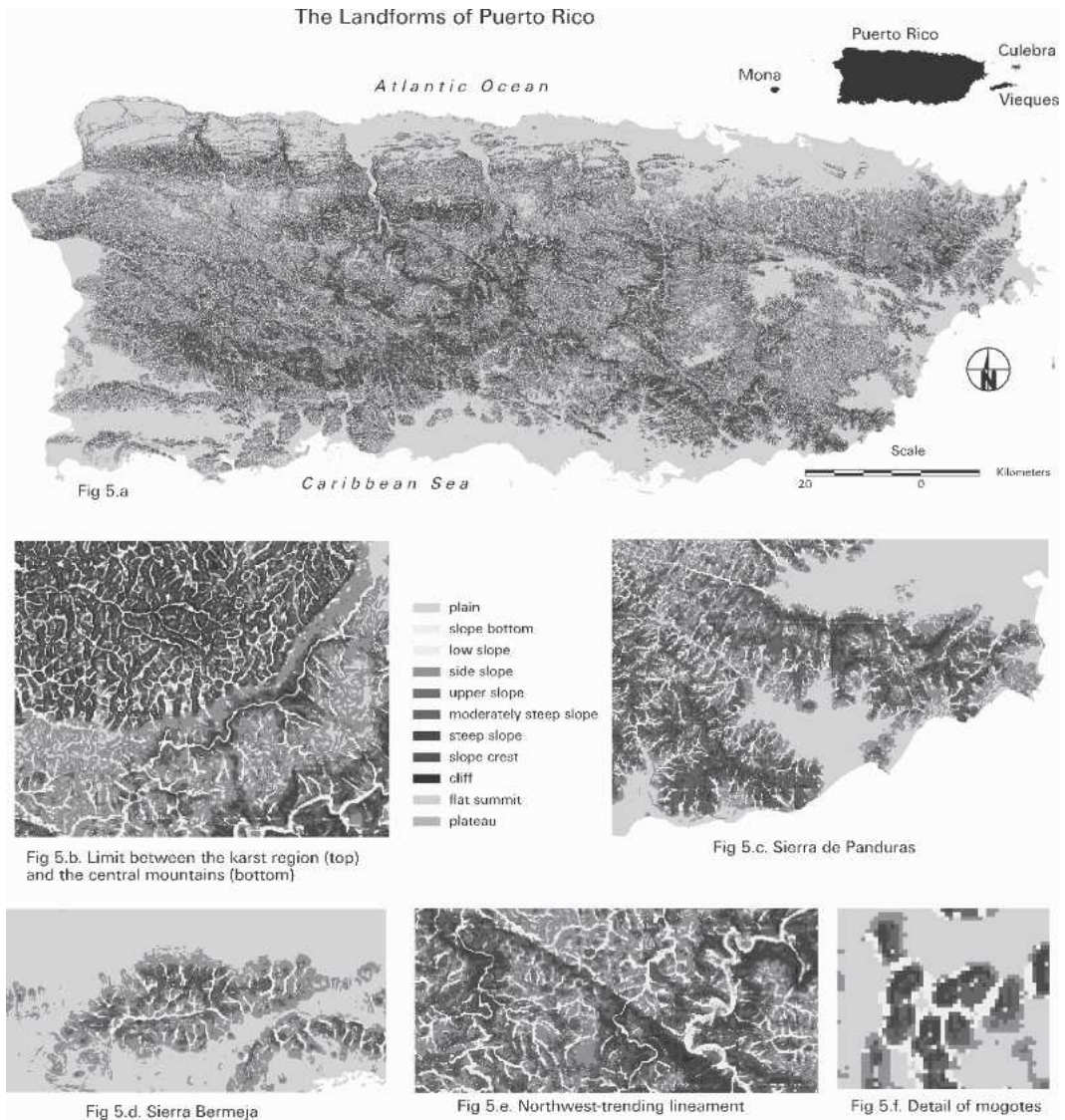
FIG. 5. View of the landform units in different regions of the island.
